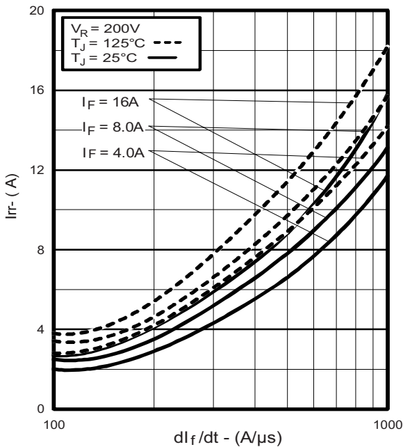
Fig. 6 - Typical Recovery Current vs. di/dt (Per Leg)
