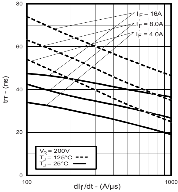
Fig. 5 - Typical Reverse Recovery Time vs. di/dt (Per Leg)
